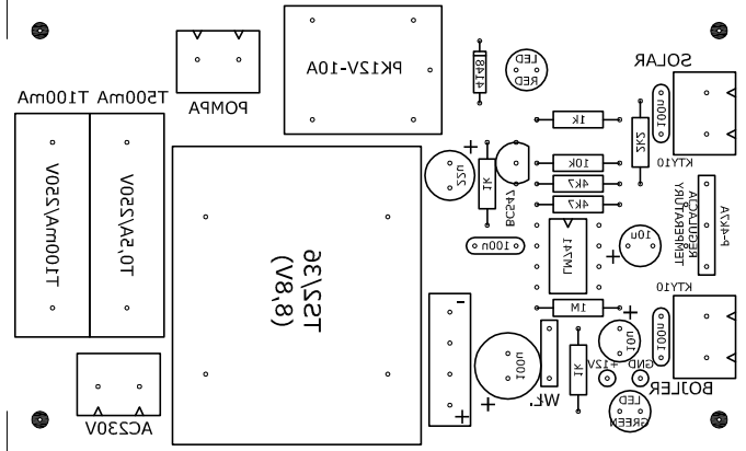
SOLAR PCB 55x90mm (TOP MIRROR)
