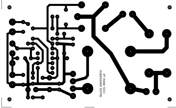
SOLAR PCB 55x90mm (BOTTOM MIRROR)
