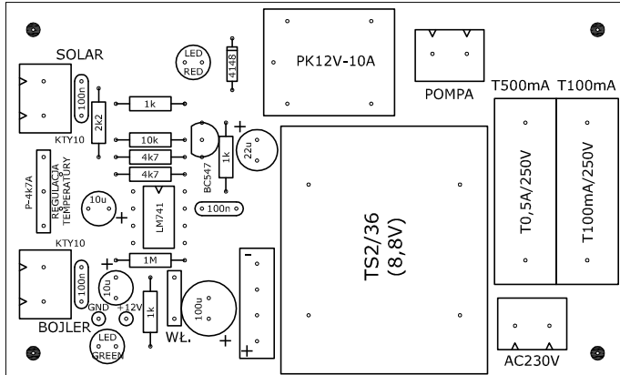
SOLAR PCB 55x90mm (TOP)
